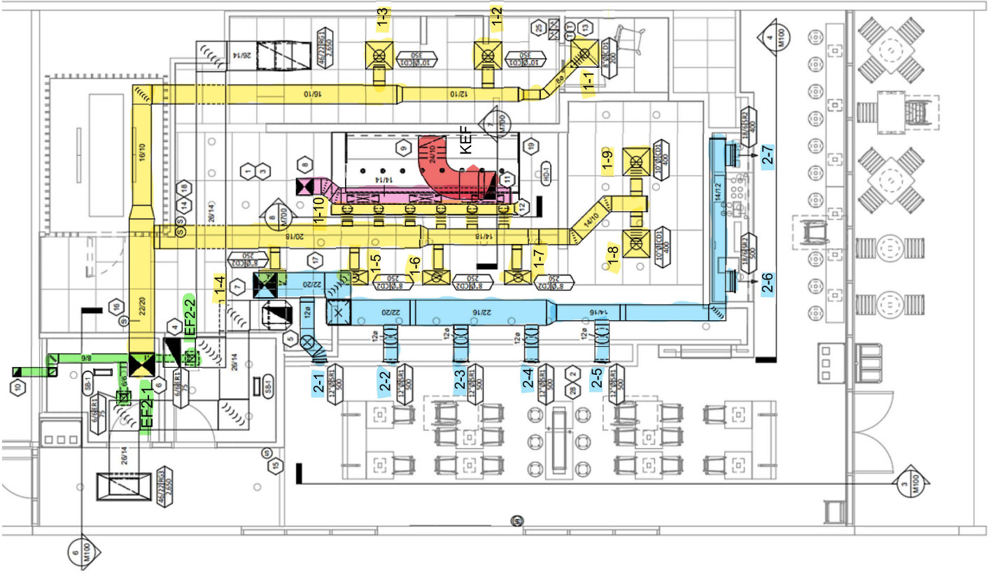
HVAC FLOOR PLAN
